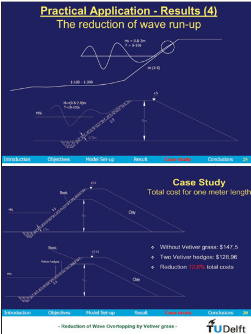
Figure 6: Wave run on the outer wall (upper) and construction cost saving with and without vetiver (lower).
